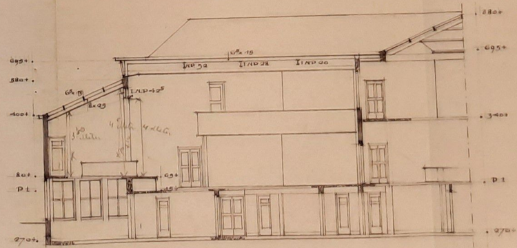
DOORSNED E B-B
